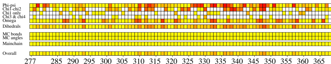
g. G-factors
