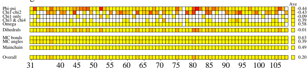
g. G-factors
