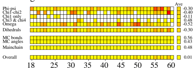
g. G-factors
